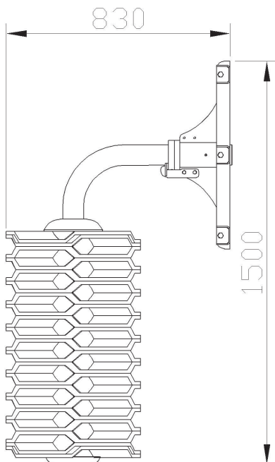
Maxi 700381246 (830 x 1500 mm)
